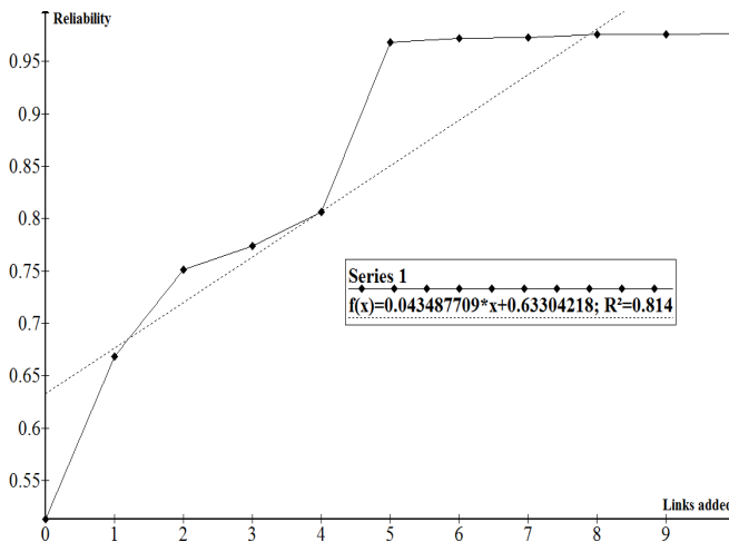
Figure 7 Reliability improvement of Network A
