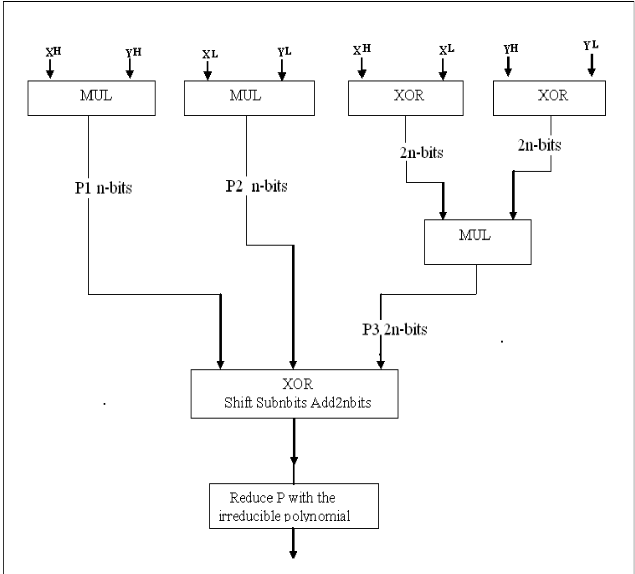
Fig-2 Hardware diagram for Karatsuba multiplication
