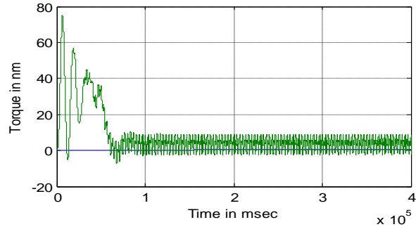
Figure.10 Torque curve of induction motor.
