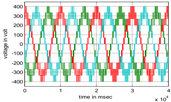
Figure 6. Three phase output line voltage of FCMLI
