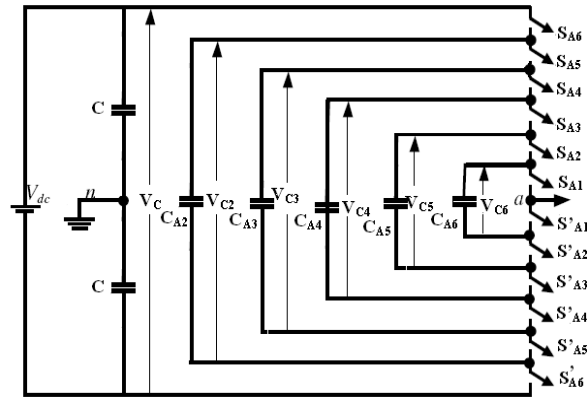
Figure 2. Phase-A leg of the seven level inverter.
