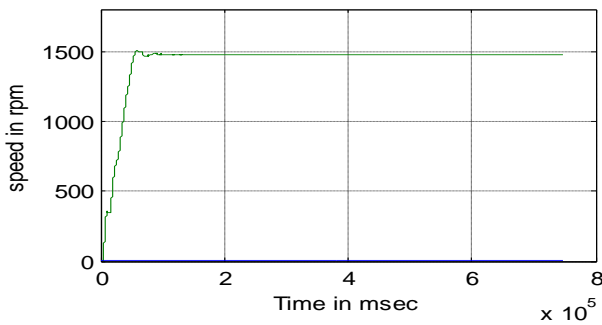
Figure.8 Speed curve of induction motor
