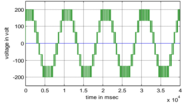
Figure 4. Phase voltage of FCMLI
