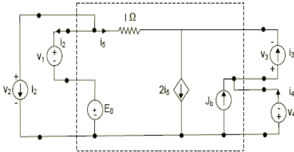
Figure1. Electrical Circuit
