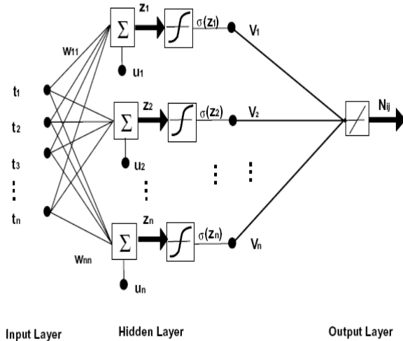
Fig. 6. Neural network architecture.
