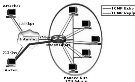
Figure 7. ICMP smurf attack
