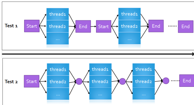
Fig. 4: Evaluation of omp_quiesce
