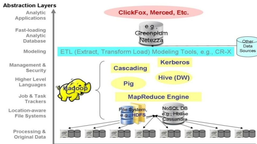
Figure 5 Various components of big data analytics
