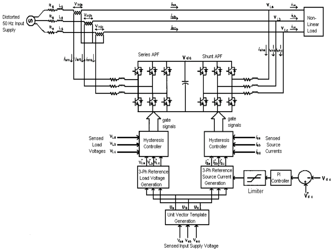
Figure.2 Overall Control Circuit Configuration of UPQC
