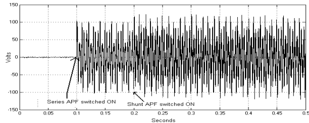
Figure. 11 Wave forms of Voltage Injected by Series APF
