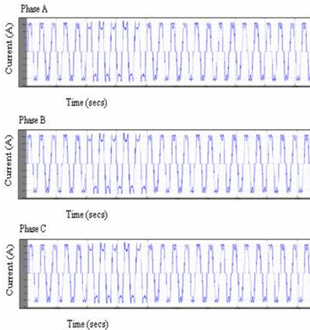
Figure. 9 Wave form of 3-Φ Source currents without UPQC for Phase A, Phase B and Phase C
