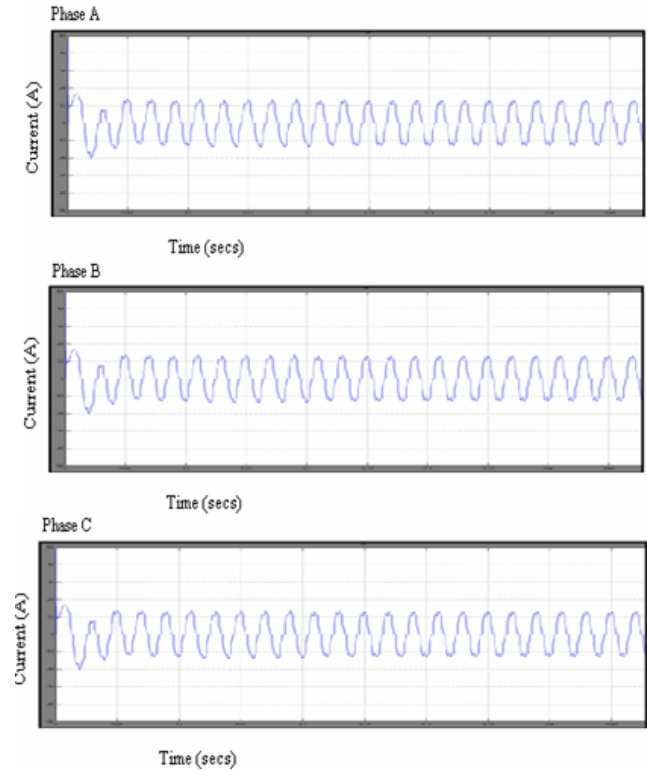
Figure. 15 Wave forms of 3-Φ Source Currents with UPQC for Phase A, Phase B and Phase C
