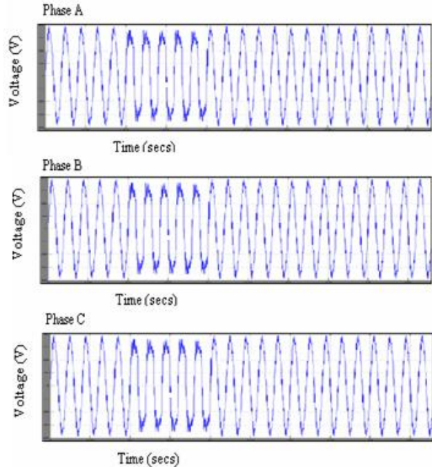
Figure.8 Wave form of 3-Φ load voltages without UPQC for Phase A, Phase B and Phase C
