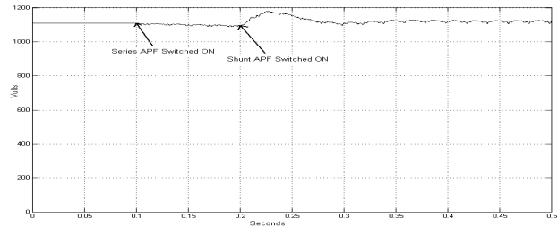
Figure. 13 Wave forms of D.C Link Voltage
