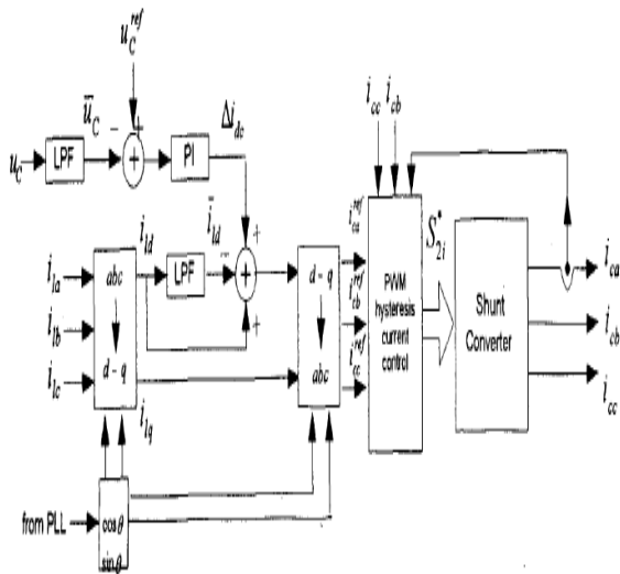
Figure.4 Control of the shunt Converter of the UPQC
