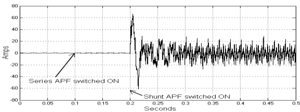
Figure. 12 Wave forms of Current Injected by Shunt APF
