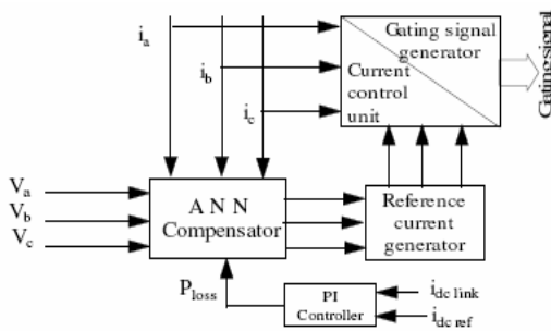
Figure.7 Block diagram of ANN-based compensator
