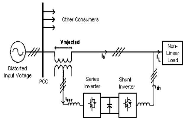
Figure.1 Basic Block Diagram of UPQC
