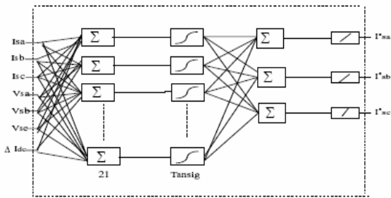
Figure.6 Network Topology of ANN
