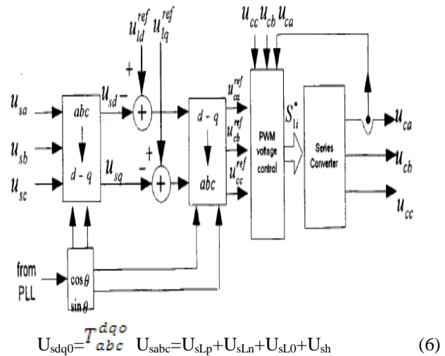
Figure.5 Control block diagram of the series converter of the UPQC
