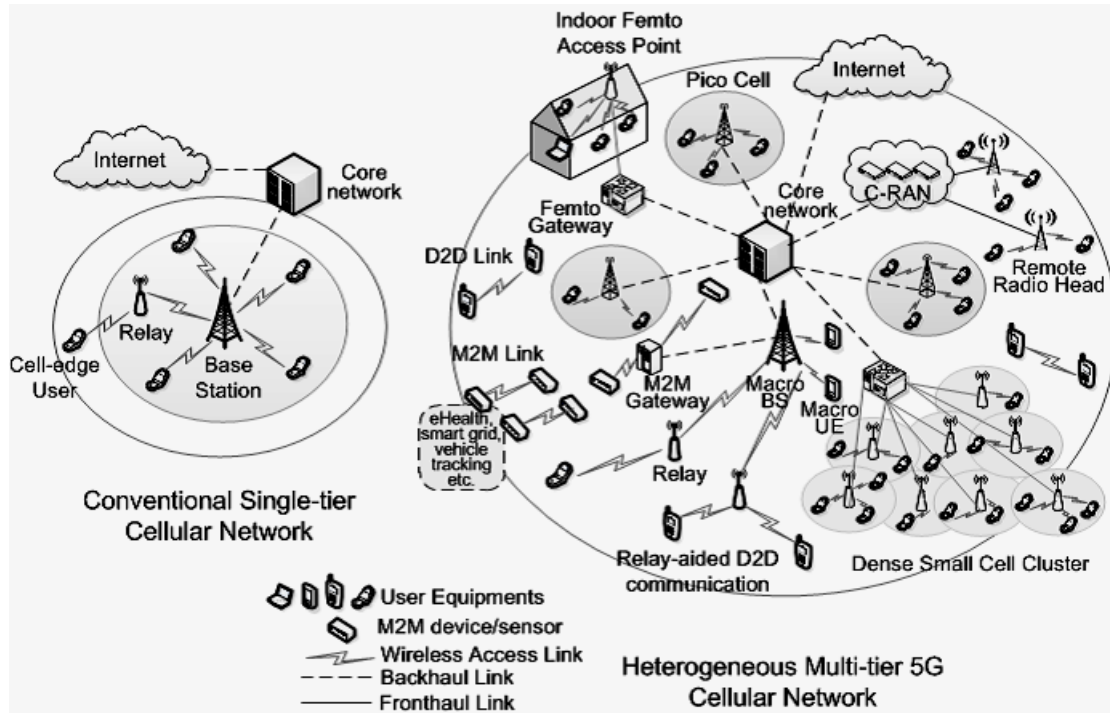
Figure 3 Heterogeneous Multi-Tier 5G Cellular Network
