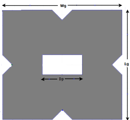
Figure 1(c). Proposed antenna design (Ground)
