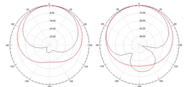
Fig 5: E- and H-plane patterns at 3.3 GHz
