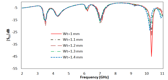
Fig 3: Return loss of antenna for variation in L-slot on Patch (Variation in "Wt")
