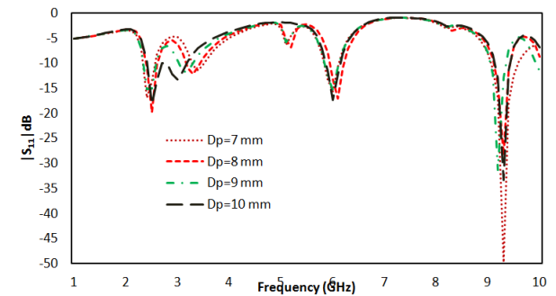
Fig 4: Return loss of antenna for variation of slot on ground plane
