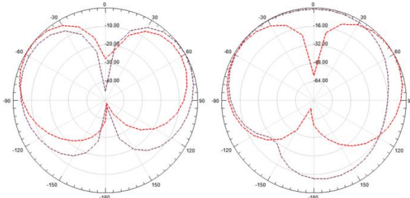
Fig 7: E- and H-plane patterns at 7.0 GHz
