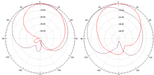
Fig 8: E- and H-plane patterns at 10.0 GHz
