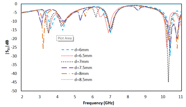
Fig 2: Return loss of antenna for variation in L-slot on Patch ( variation in "d")
