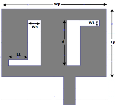
Figure 1(b). Proposed antenna design (Patch)
