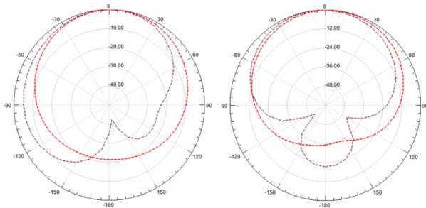
Fig 6: E- and H-plane patterns at 4.3 GHz
