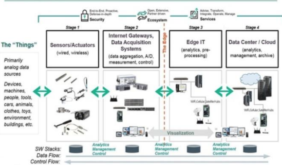
Fig.2: Stages of IoT Architecture [12]
