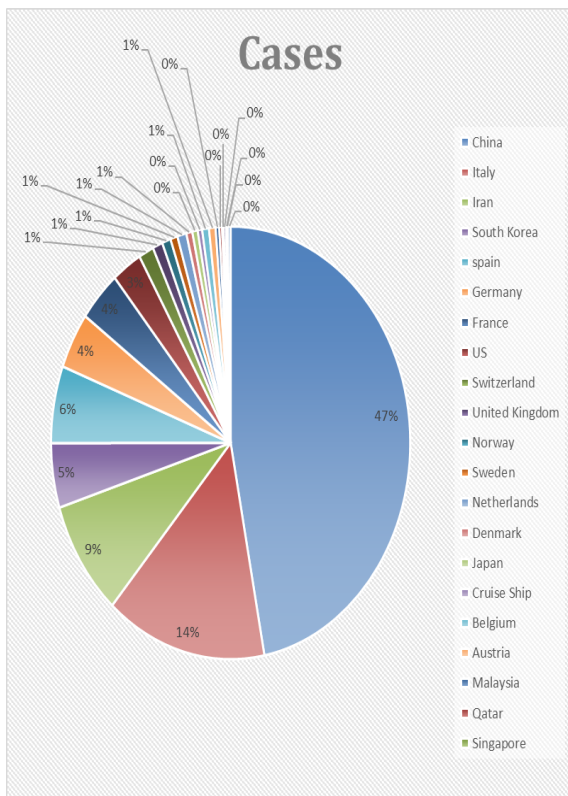
Fig 1: Estimation of the cases due to COVID-19 all over the world.
