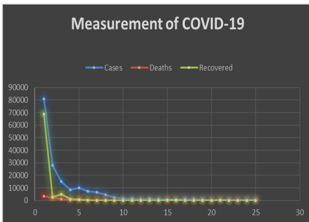
Fig 2: Measurement of COVID-19 (cases, deaths and recovered)
