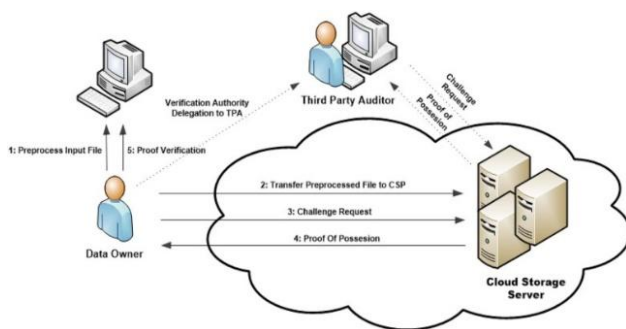
Fig 4 : Data Integrity using Third Party Auditor [35]
