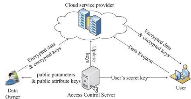
Fig. 6: Attribute Based Encryption (ABE)[35]
