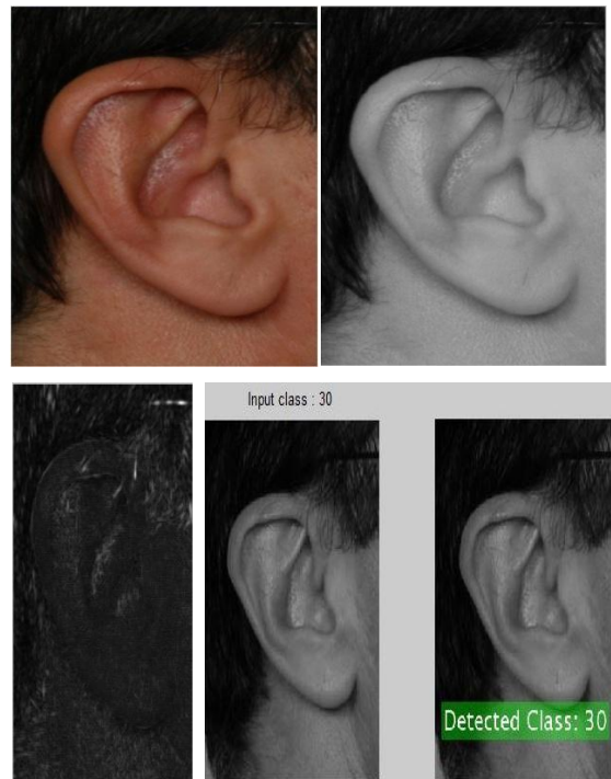
Fig 4: Implementation results
