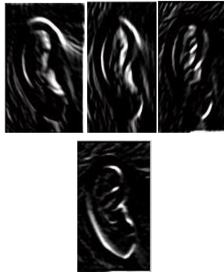
Fig3: Gabor outputs
