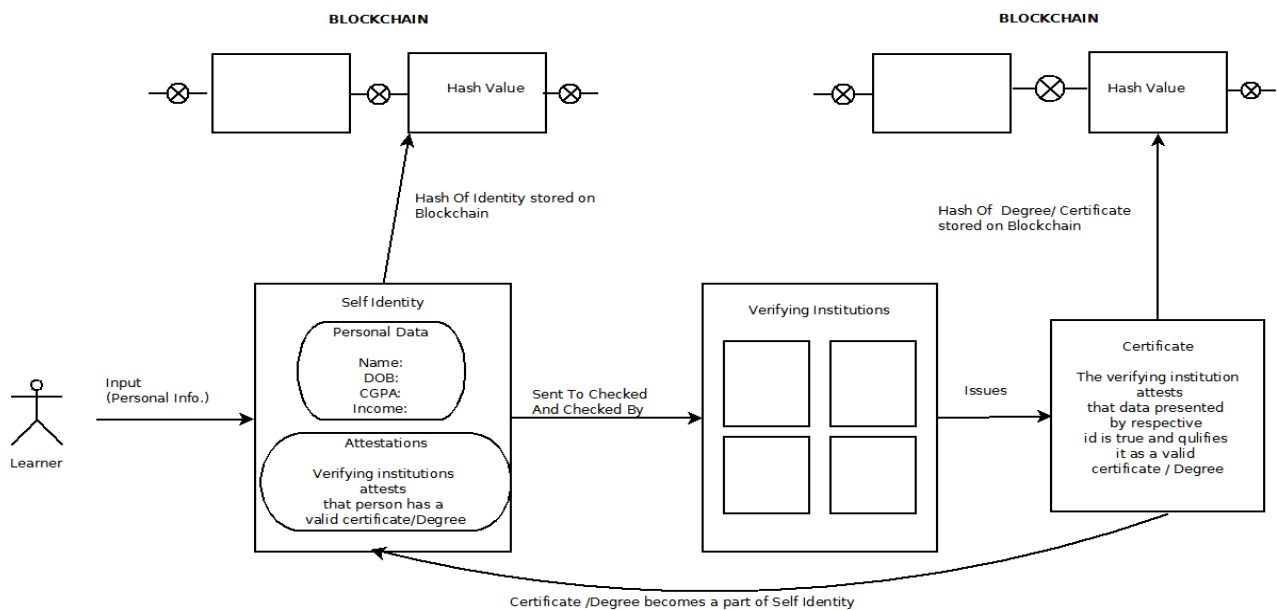
Fig 1: Digital certification overview
