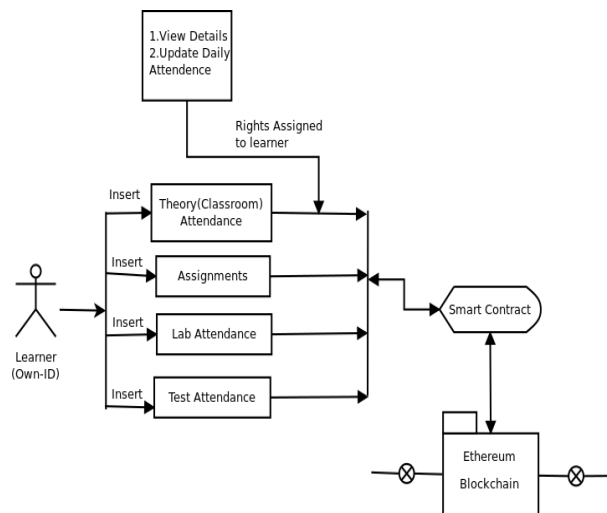
Fig. 2 Learner's module on blockchain
