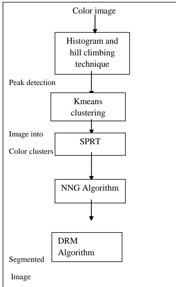
Fig 1.Flow of System
