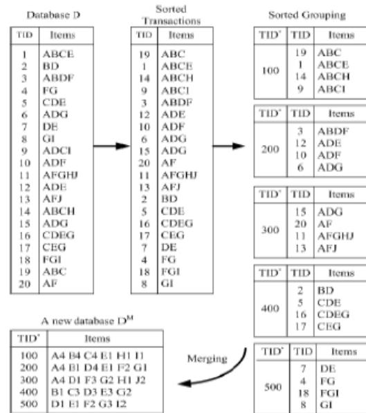
Fig 2: An example of sort grouping
