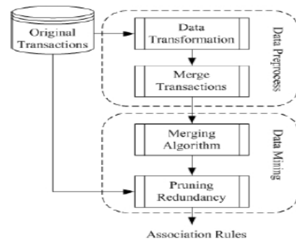
Fig 1: An overview of the Merged Transaction Algorithm
