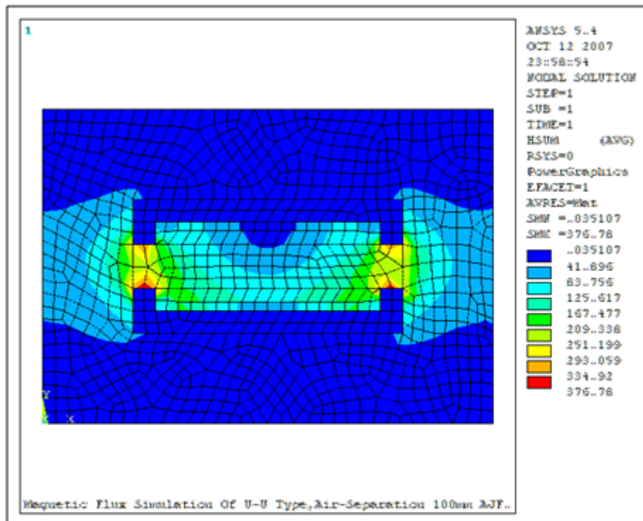
Fig.11 : Simulated distribution of contours plot of magnetic field intensity H.sum of U-U type core
