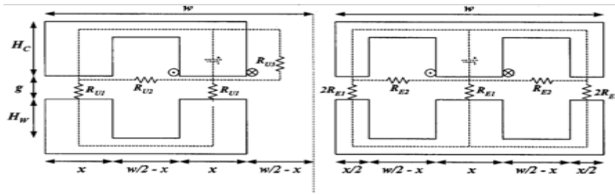
Fig.2: Core shape and the reluctances of the U-U type and E-E type
