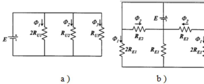
Fig.3: Equivalent magnetic circuit of (a) U-U type (b) E-E type
