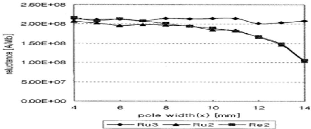
Fig.4 Reluctances of the magnetic circuit (RU2,RU3,RE2).
