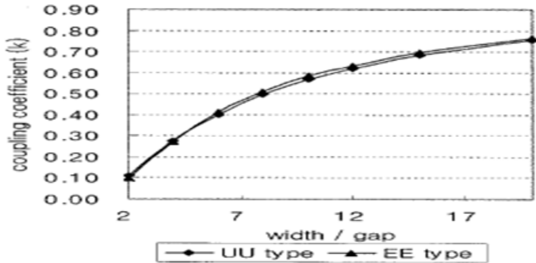
Fig.6: Coupling coefficient K as a function of the ratio (w/g) of the width (w) and the gap length (g).
