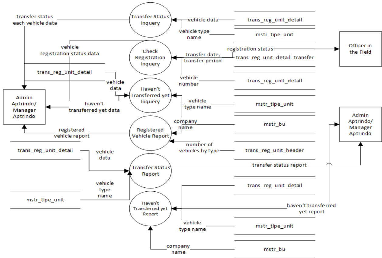
Fig 6. Data Flow Diagram (Inquiry / Report)
