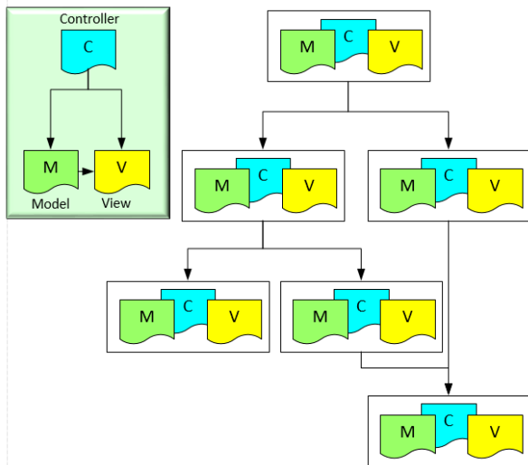
Fig 2: HMVC Concept
