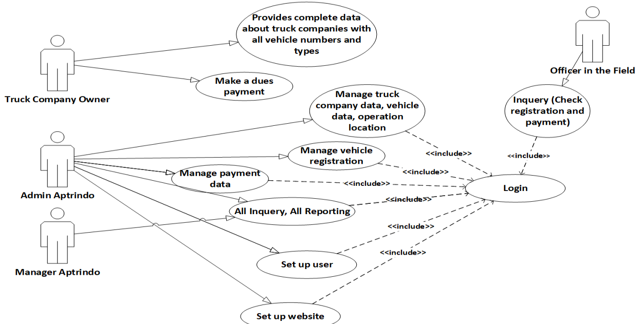
Fig 4. UseCase Diagram
