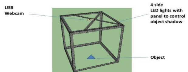
Fig. 1. Hardware of CV Cube
