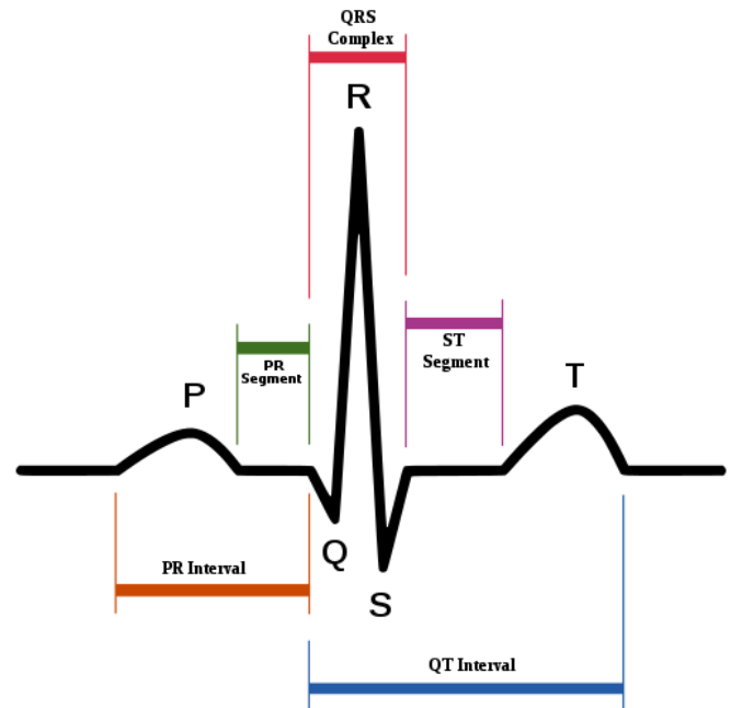
Fig1: Normal ECG [2]
