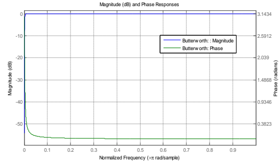
Fig2: Magnitude Response & Phase Response of Butterworth filter
