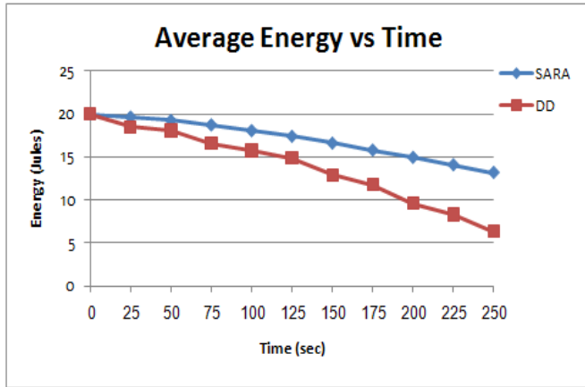
Fig 2: Calculation of delay Due to increase of source
