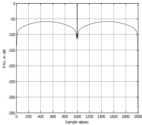
Fig 2: PSL of Amplitude weighting (Blackman)
