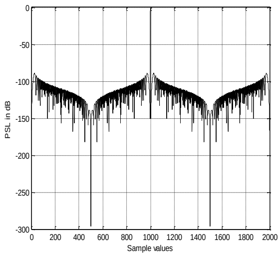
Fig 4: Woo Filter form 2
