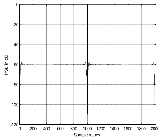
Fig 3: PSL of Woo Filter
