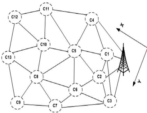
Fig. 2. Neighboring cluster-heads.
