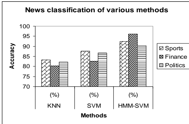
Figure 3. Graphical representation of classification accuracy of various methods
