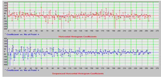
Figure 6 Hadamard Coefficients of Horizontal pixel distribution (Upper Plot) and their sequenced arrangement (Lower Plot) of the signature mentioned in Figure 3
