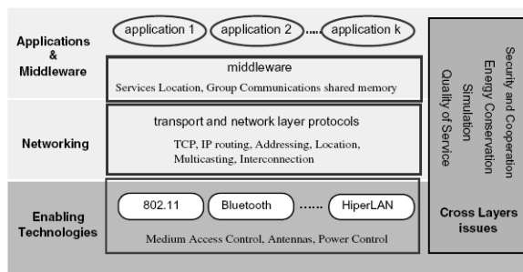
Fig 3. MANET Architecture
