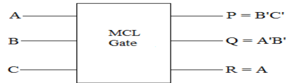
Fig 14: MCL gate
