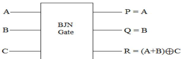
Fig 13: BJJ gate
