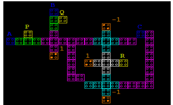
Fig 23: Simulated design of BJK gate
