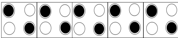
Fig 2: QCA wire
