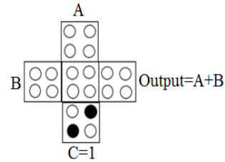
Fig 4: Majority voter as 2-input AND gate and 2-input OR gate
