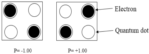
Fig 1: Four dotted QCA cell
