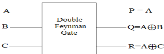
Fig 8: Double Feynman gate
