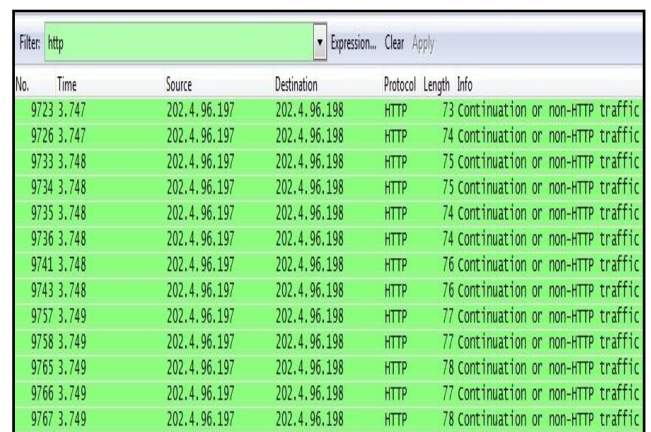
Fig.7 Received HTTP packets with partial data captured from the victim web server
