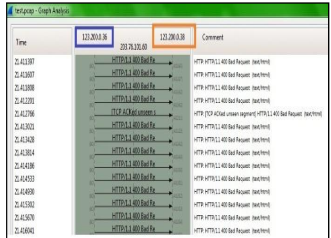
Fig. 3 400 HTTP bad requests to the attacking server 123.200.0.38 from the victim 123.200.0.36
