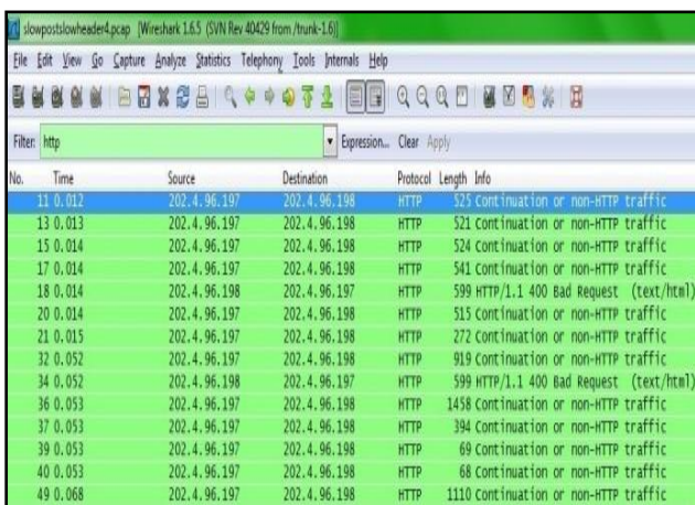
Fig.5 Received partial HTTP packets captured from victim Web server
