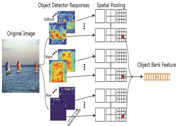
Fig 12 Object Detector Responses
