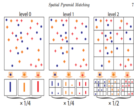
Fig 11 Spatial Pyramid Matching
