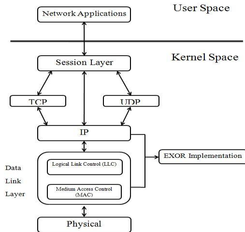
Figure 3. Layered Architecture – EXOR Implementation
