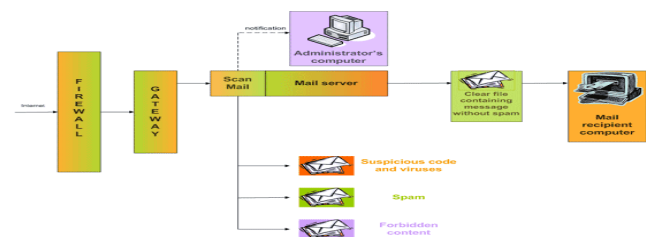
Figure 1. Spam Filter Architecture
