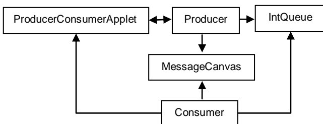
Fig 1: Simulator Classes
