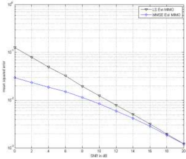
Figure 6. MSE for LS/MMSE Estimators to MIMO OFDM Systems
