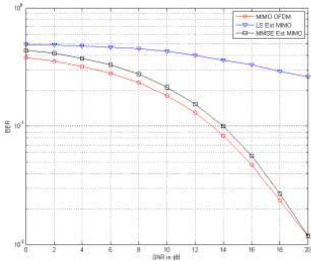
Figure 10. BER plot for comb type MIMO OFDM with LS/MMSE Estimators
