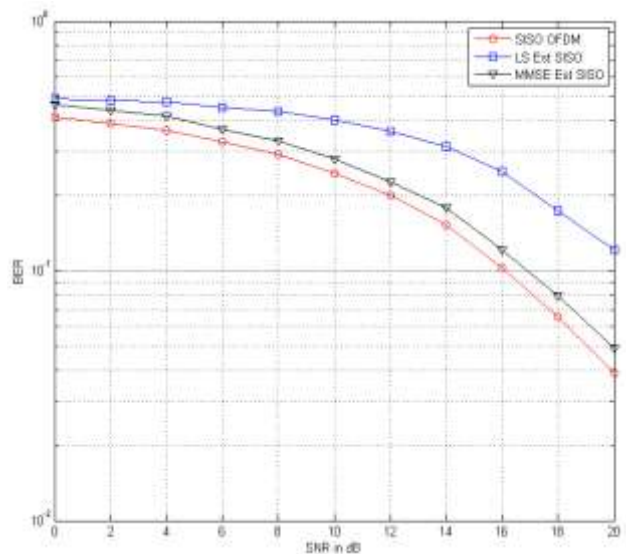
Figure 9. BER plot for comb type SISO OFDM with LS/MMSE Estimators
