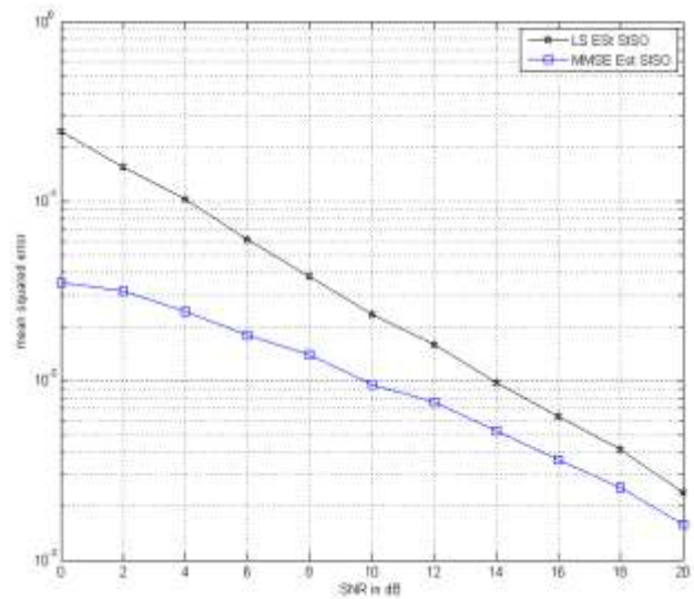
Figure 5. MSE for LS/MMSE Estimators to SISO OFDM Systems
