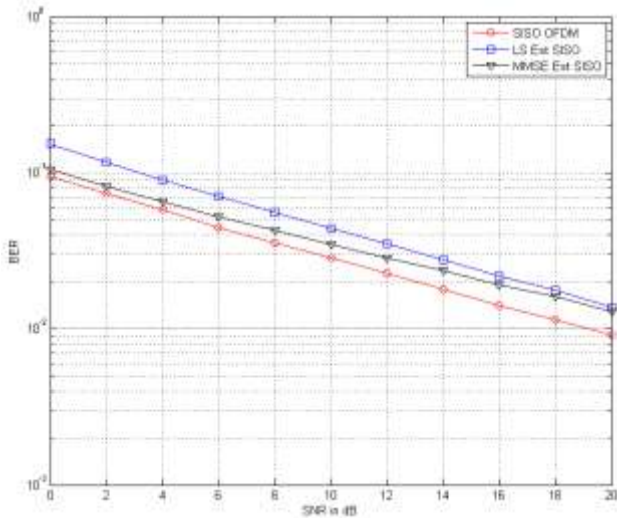
Figure 7. BER plot for Block type Pilot based SISO OFDM with LS/MMSE Estimators
