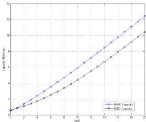
Figure 4. Capacity vs. SNR for SISO/MIMO OFDM Systems
