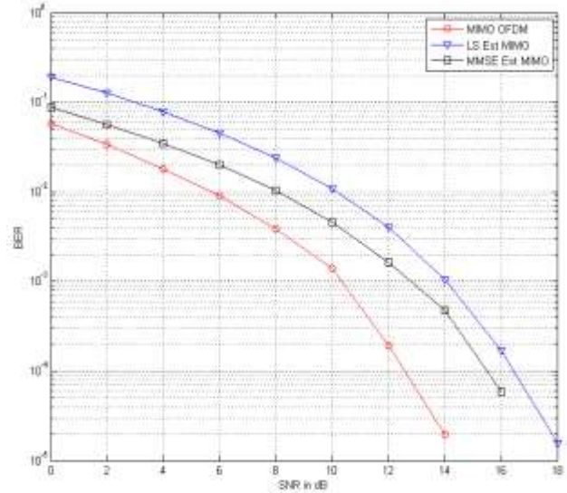
Figure 8. BER plot for Block type pilot based MIMO OFDM with LS/MMSE Estimators
