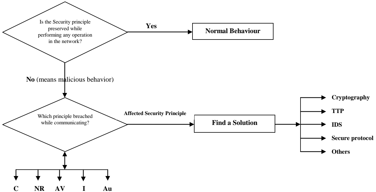
Fig.3. Defined Algorithm for Normal & Malicious Behavior of a Node
