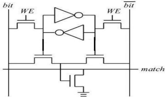
Fig 2: Basic XNOR CAM cell
