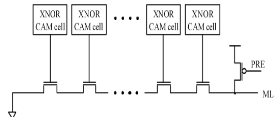
Fig 6: NAND CAM Array
