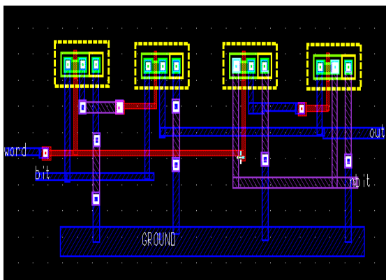
Fig 9: 4T CAM Cell layout in 0.18 um standard CMOS Technology.
