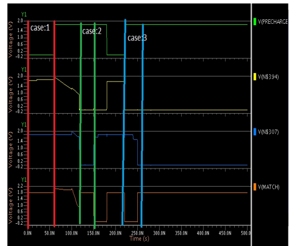
Fig 8. Simulation results of HYBRID CAM
