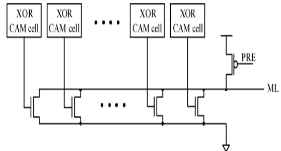
Fig 5: NOR type CAM Array
