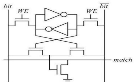
Fig 1: Basic XOR CAM cell
