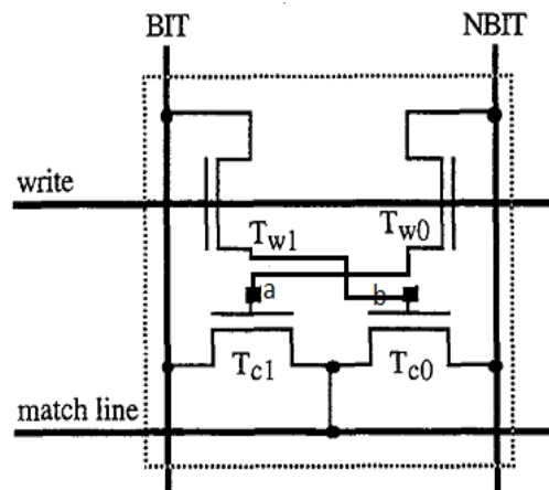
Fig 4: 4T XNOR CAM cell
