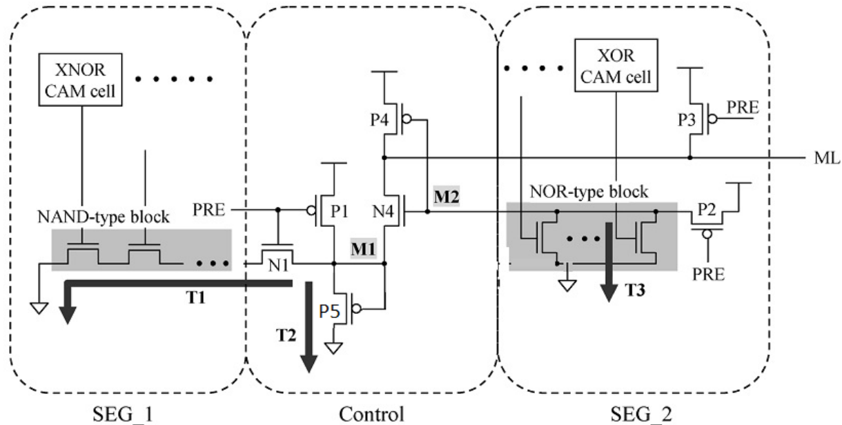
Fig 7: HYBRID CAM Structure [Ref 7]
