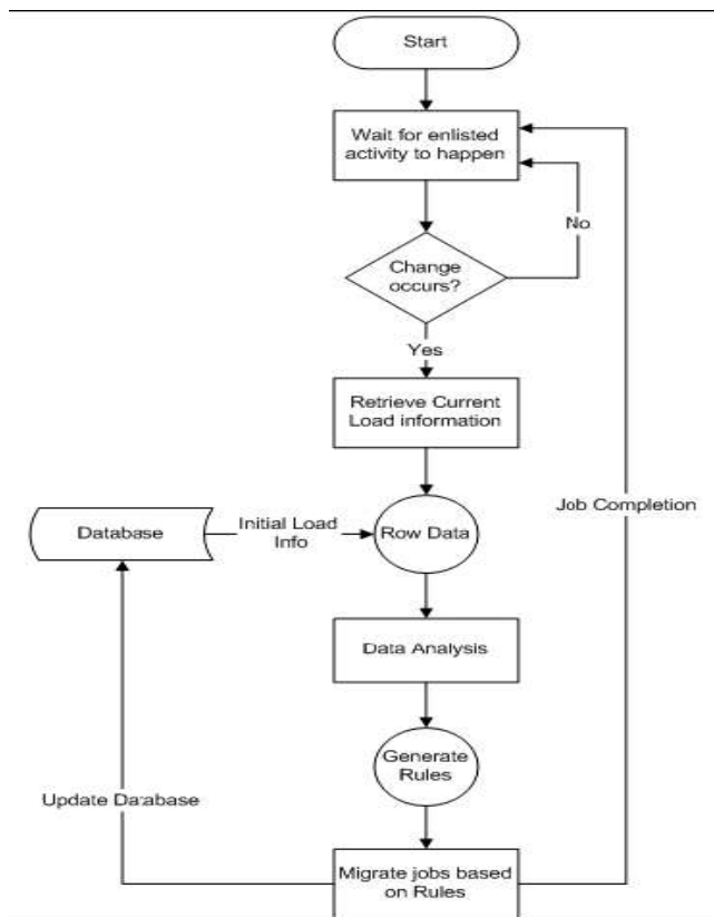
Figure 3. System Architecture
